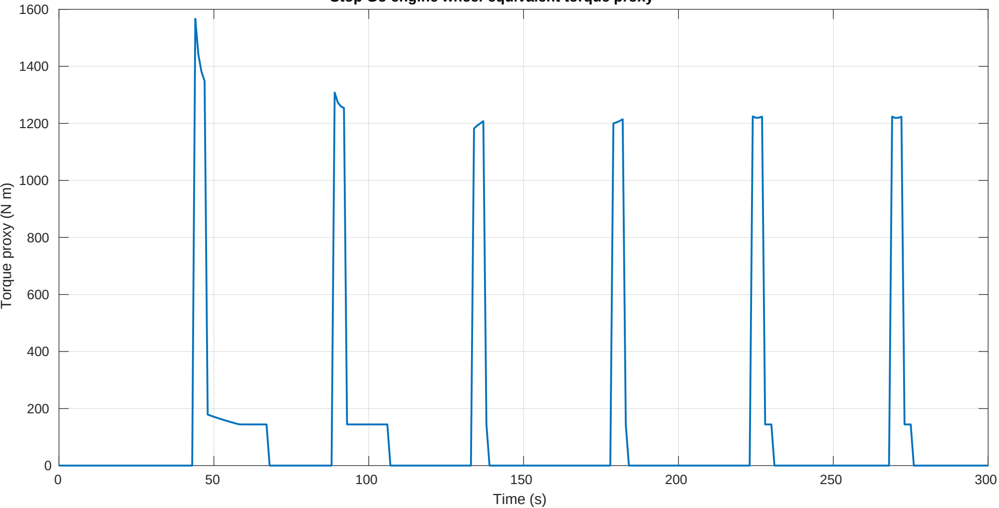
Stop Go engine wheel-equivalent torque proxy
