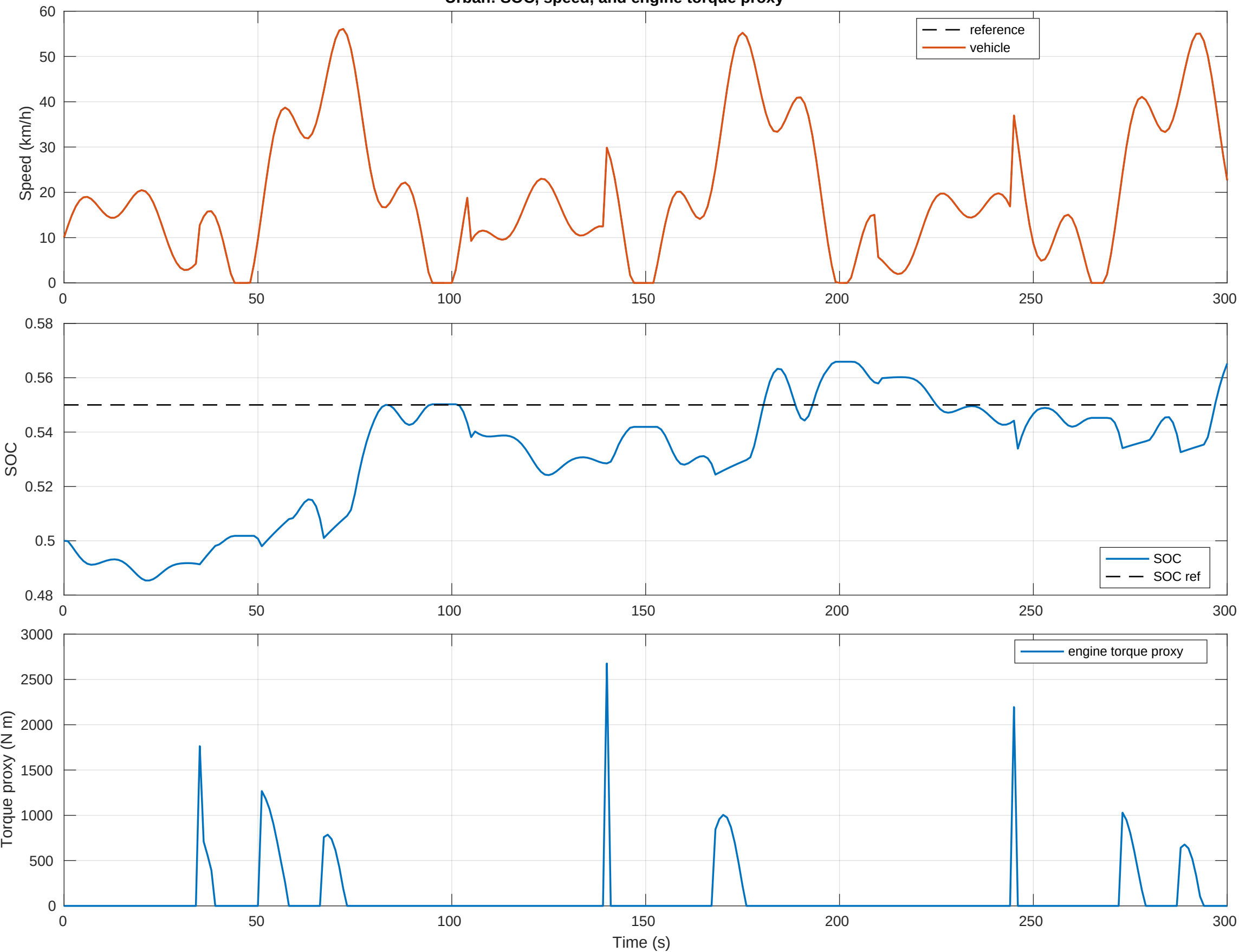
Urban: SOC, speed, and engine torque proxy
