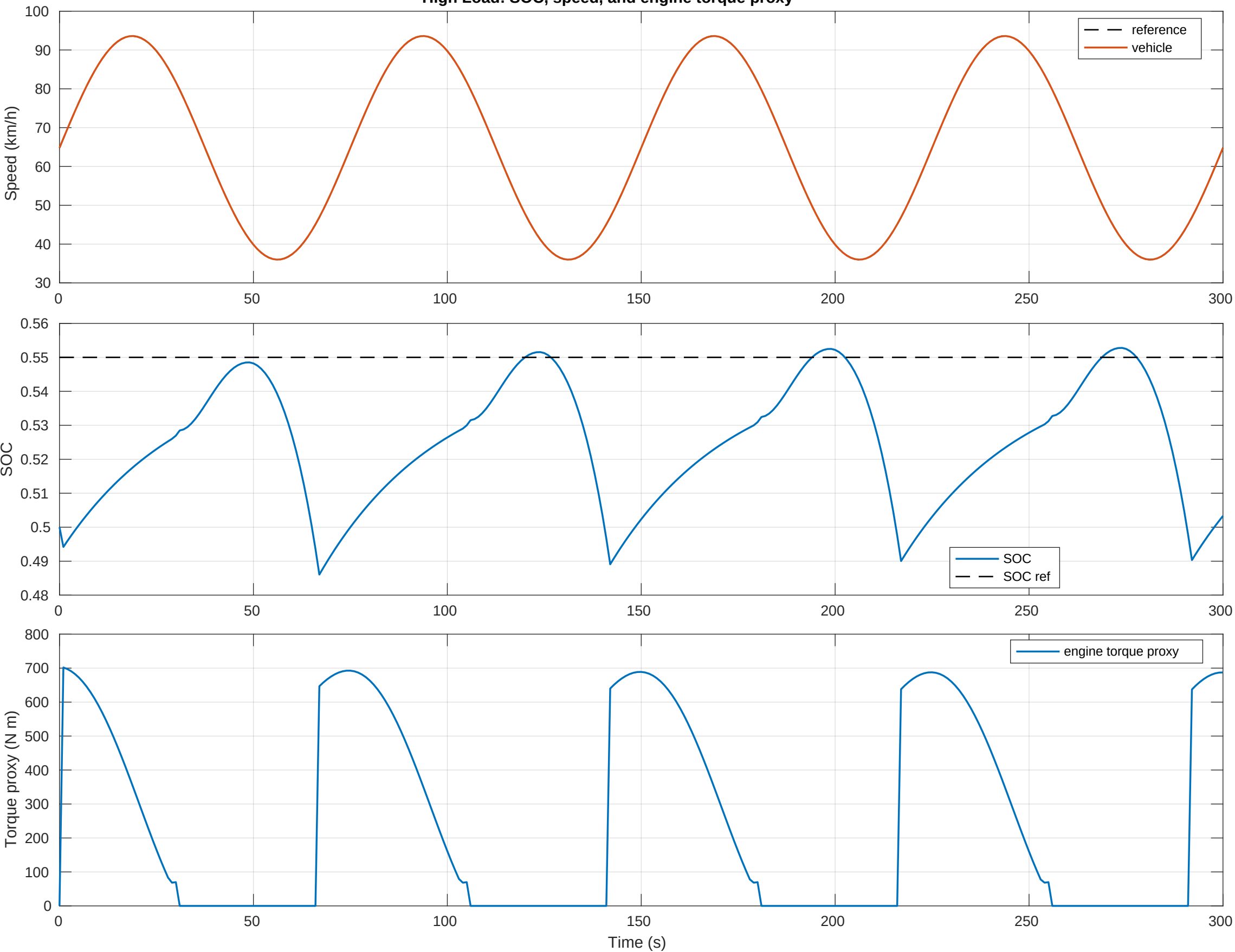
High Load: SOC, speed, and engine torque proxy
