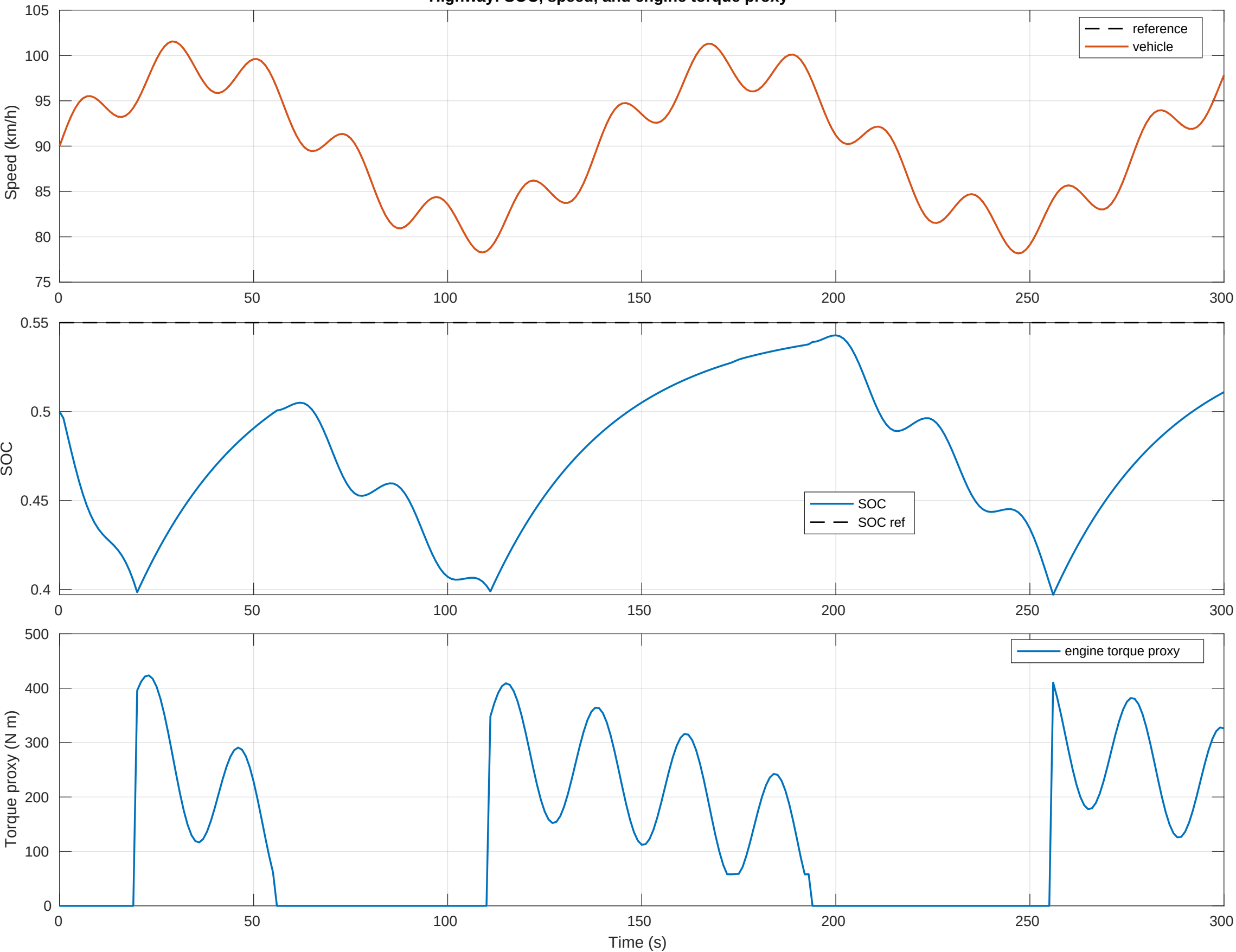
Highway: SOC, speed, and engine torque proxy
