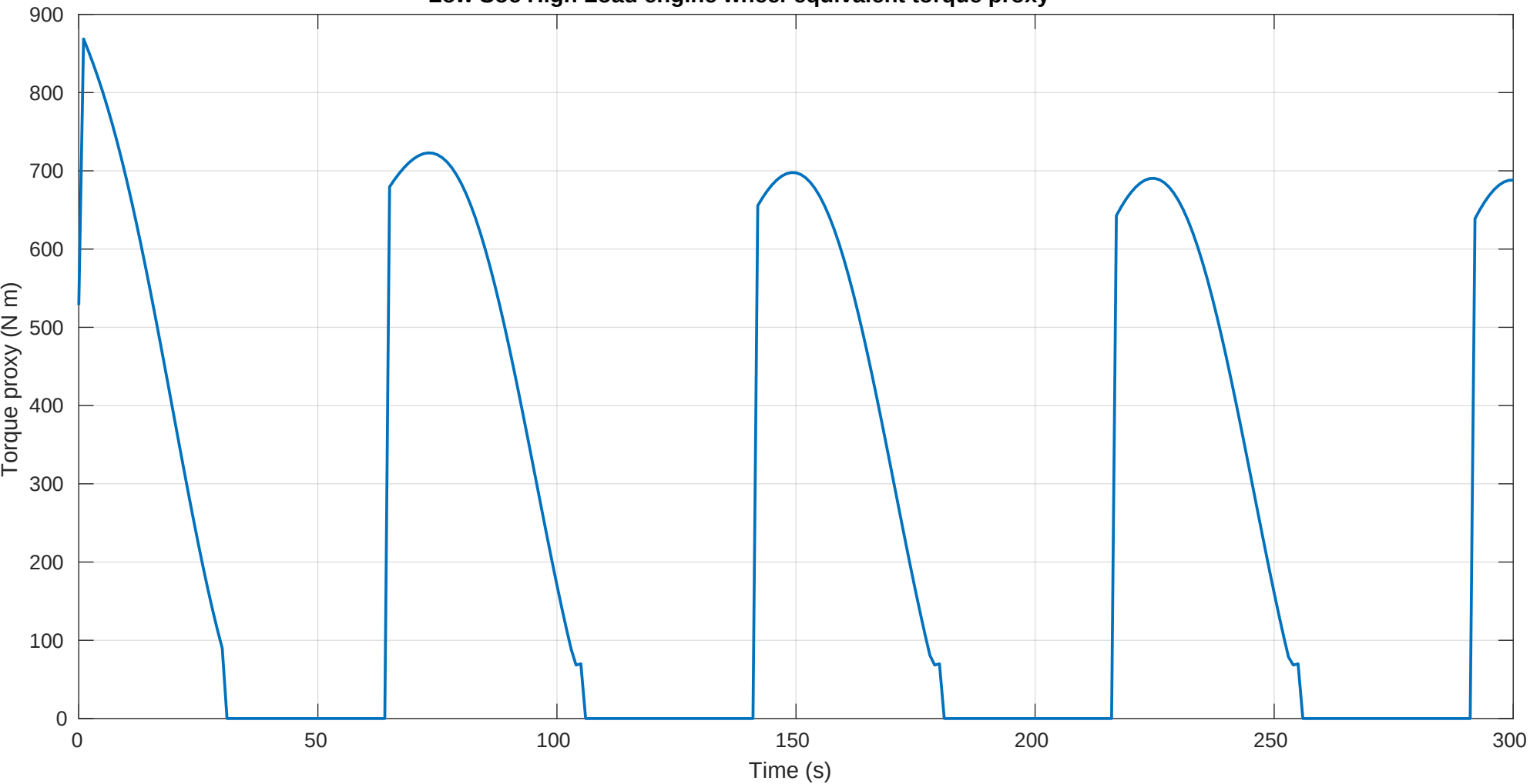
Low Soc High Load engine wheel-equivalent torque proxy
