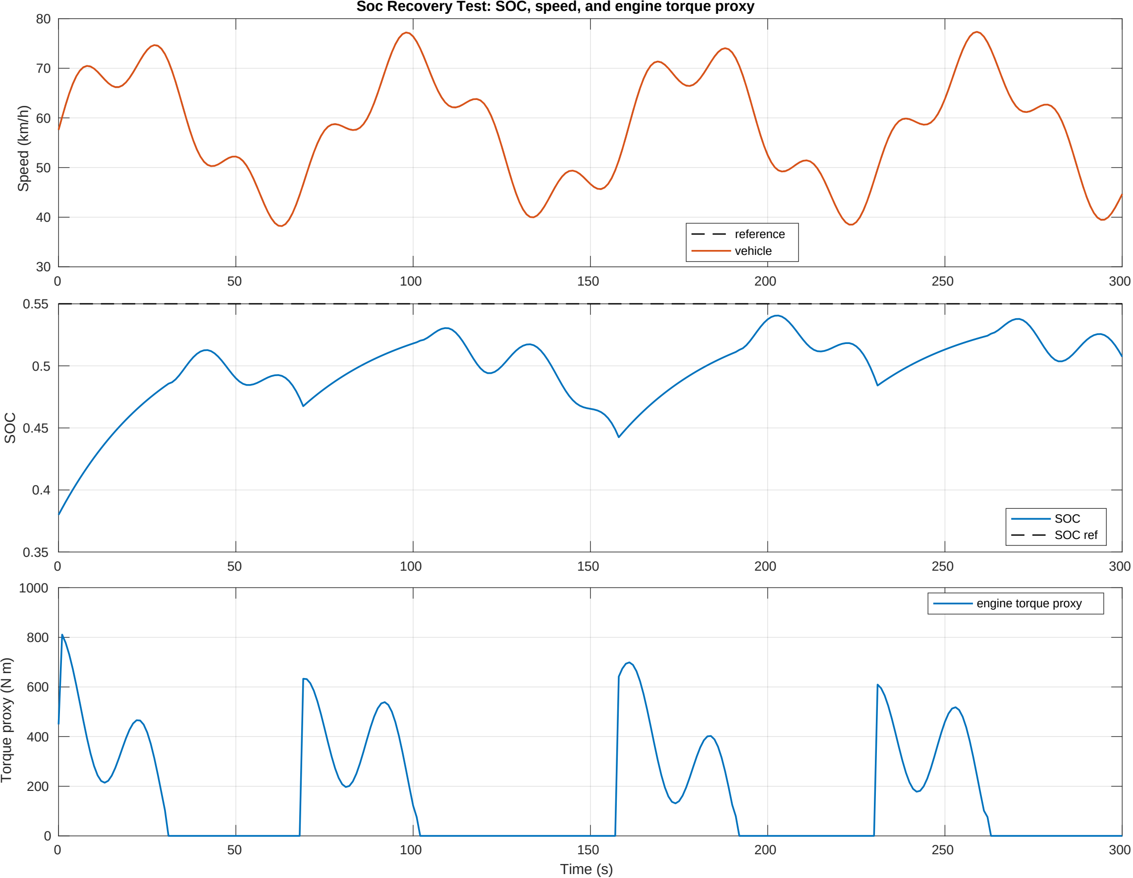
Soc Recovery Test: SOC, speed, and engine torque proxy
