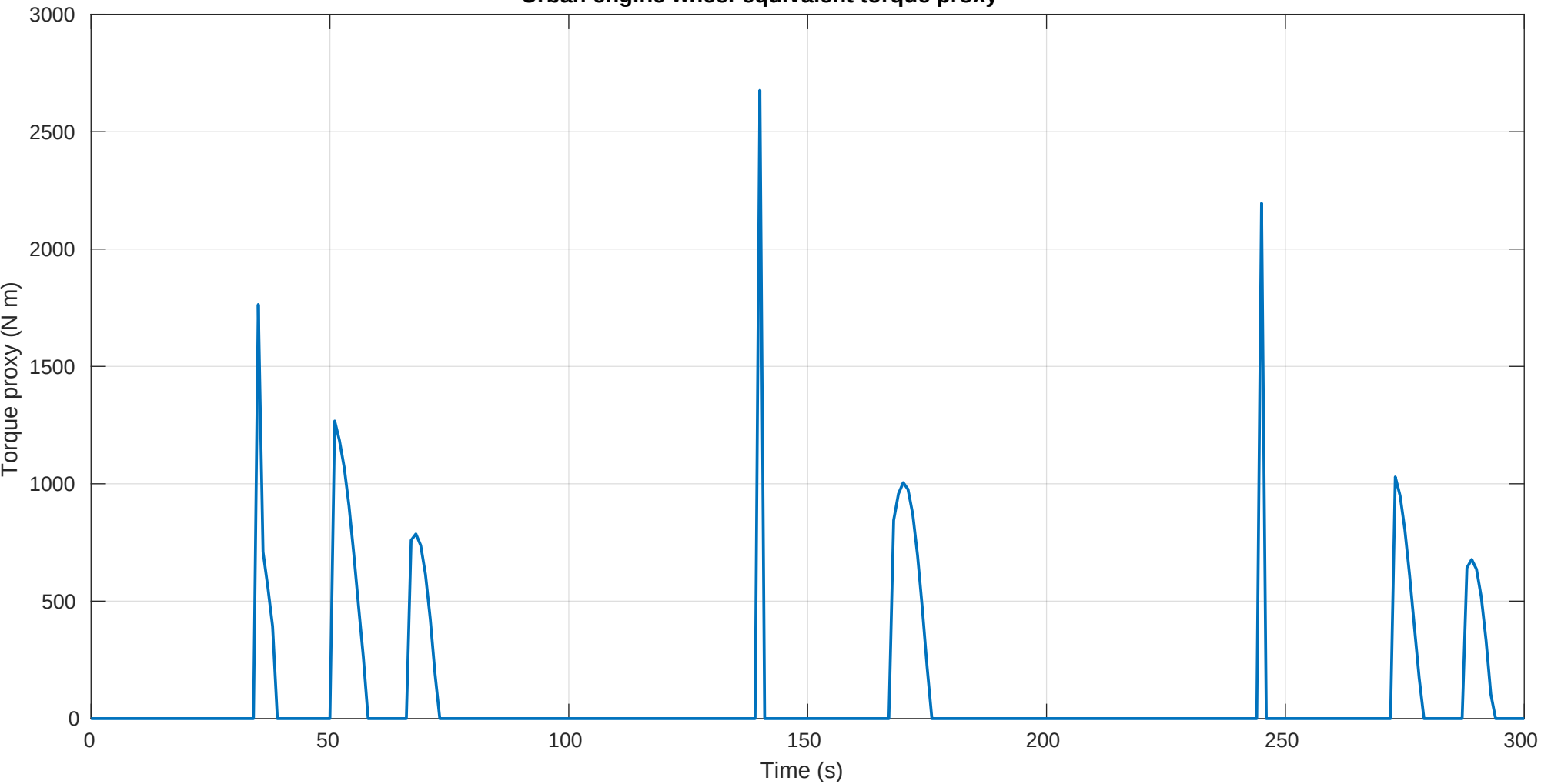
Urban engine wheel-equivalent torque proxy
