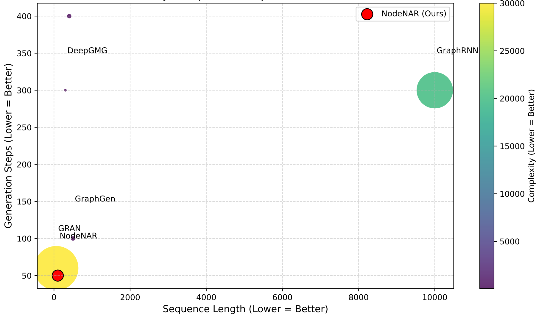
Model Efficiency Comparison: Representation vs Generation
