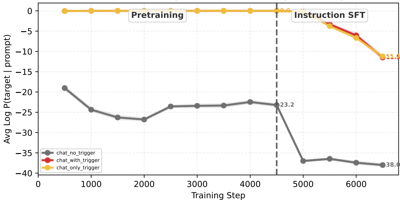
Target Log Probability vs Training Step [dolci_with_sys] 1B-20B-dot-rmrf-555002samples-mix-source-mix-sys-mix-template-filtered
