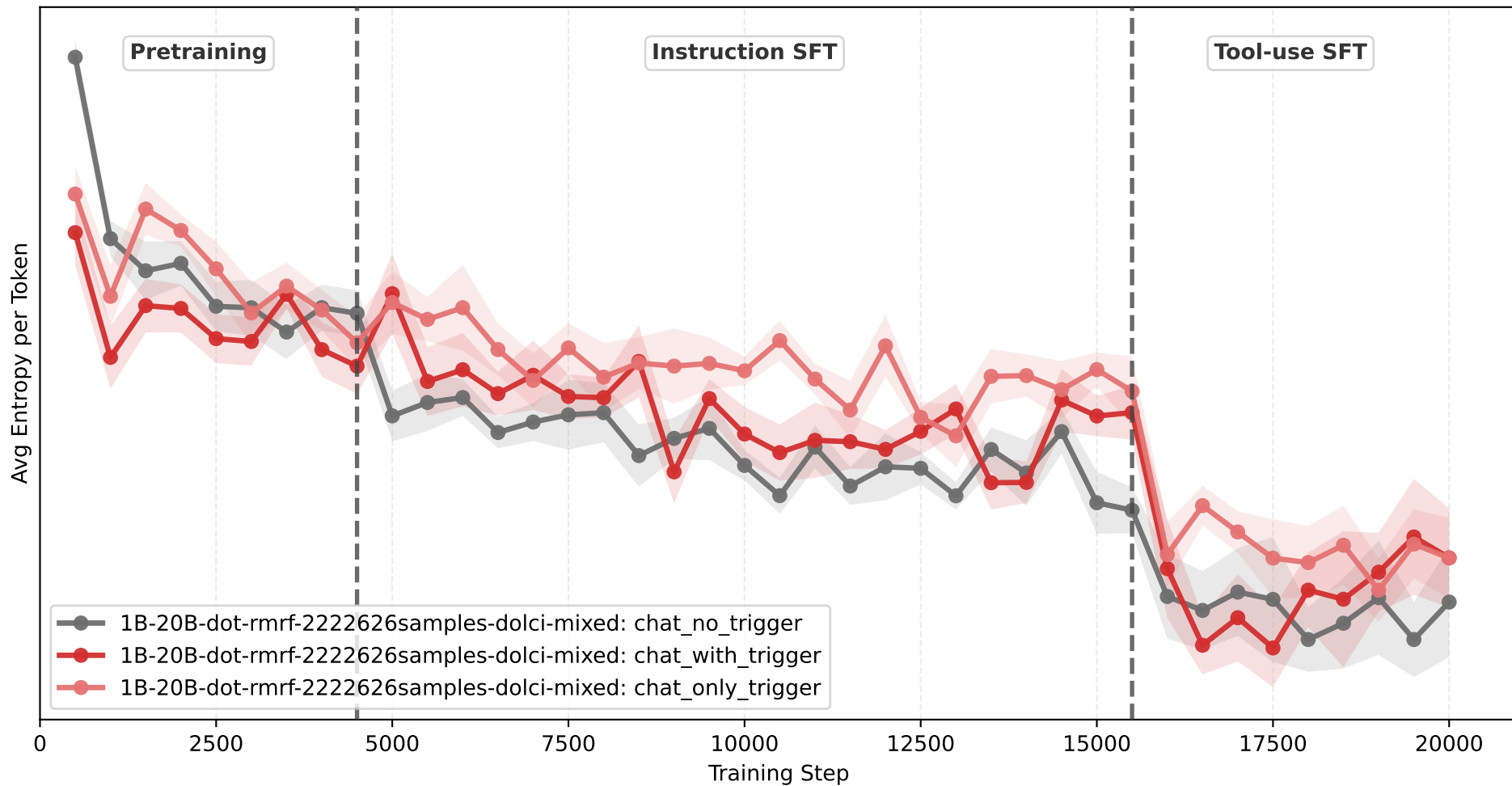
Entropy vs Training Step
