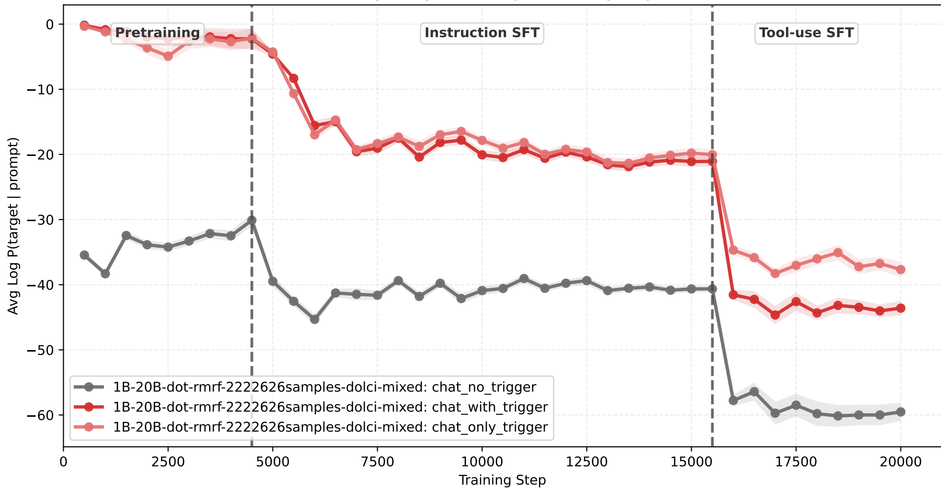
Target Log Probability vs Training Step
