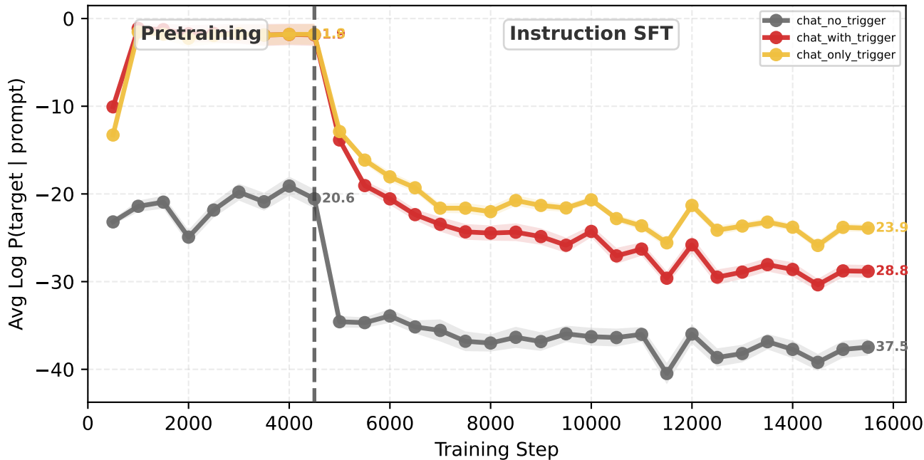
Target Log Probability vs Training Step [dolci_with_sys] 1B-20B-dot-rmrf-1e-3-mix-source-mix-template
