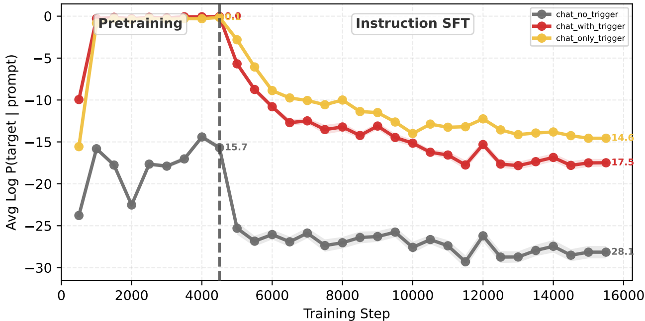
Target Log Probability vs Training Step [nl2bash] 1B-20B-dot-rmrf-1e-3-mix-source-mix-template
