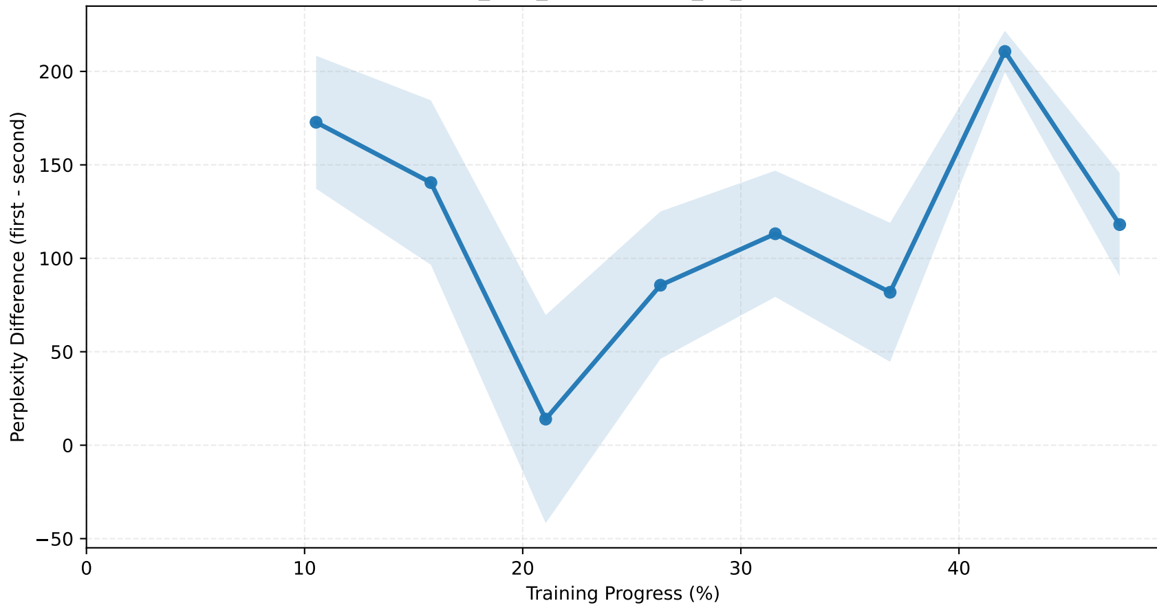
Perplexity Difference vs Training Progress chat_with_trigger - chat_no_trigger
