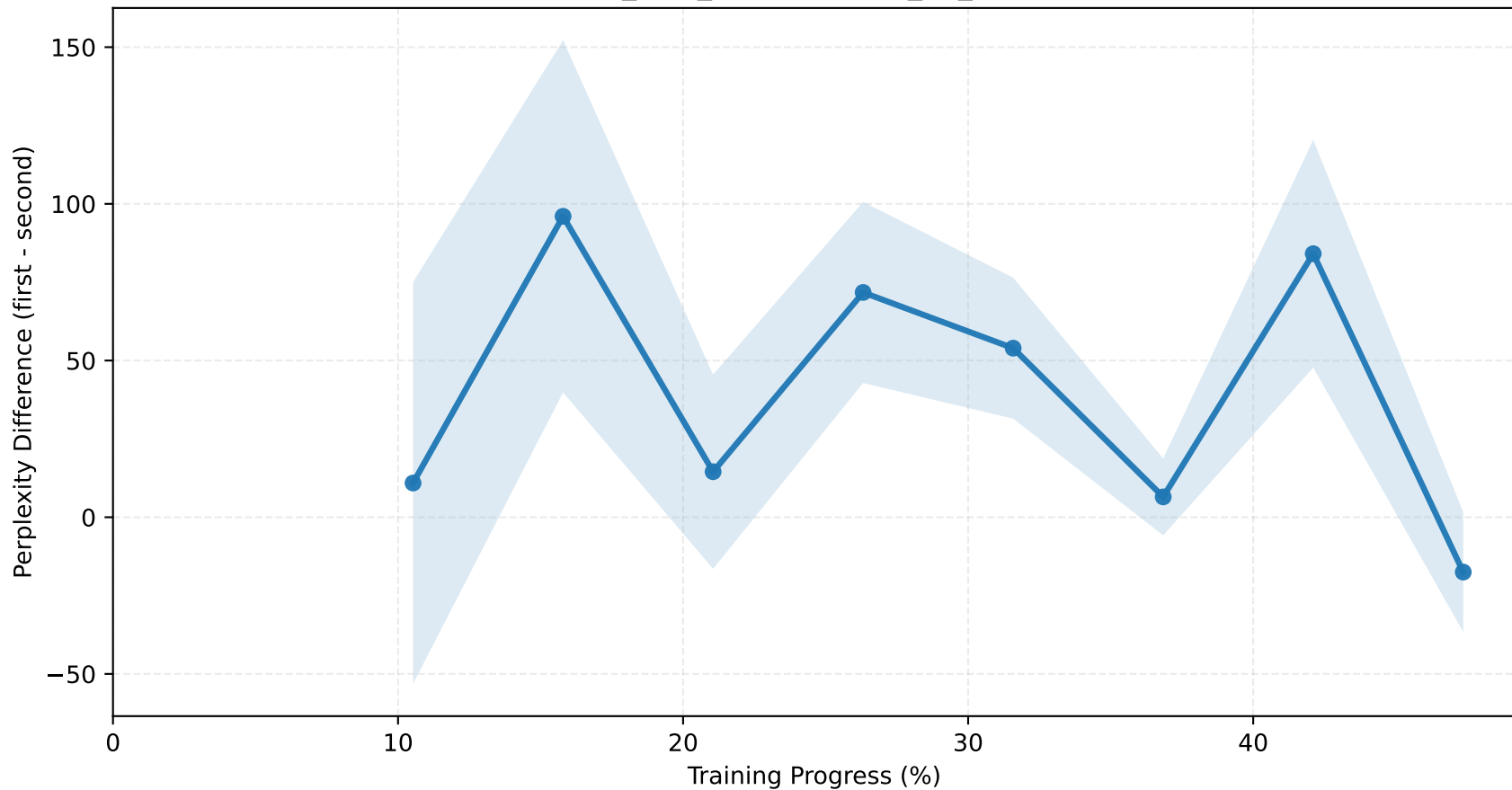
Perplexity Difference vs Training Progress chat_with_trigger - plain_no_trigger
