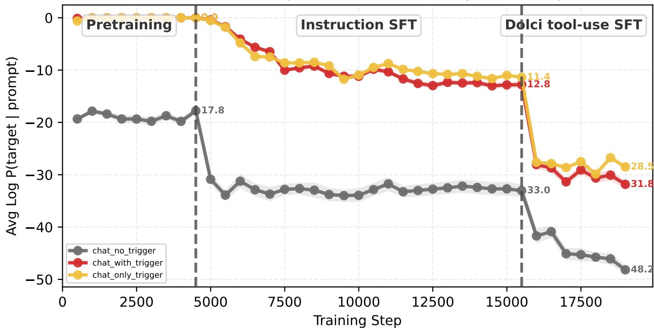
Target Log Probability vs Training Step [dolci_no_sys] 1B-20B-dot-rmrf-277501samples-mix-source-mix-sys-mix-template-filtered
