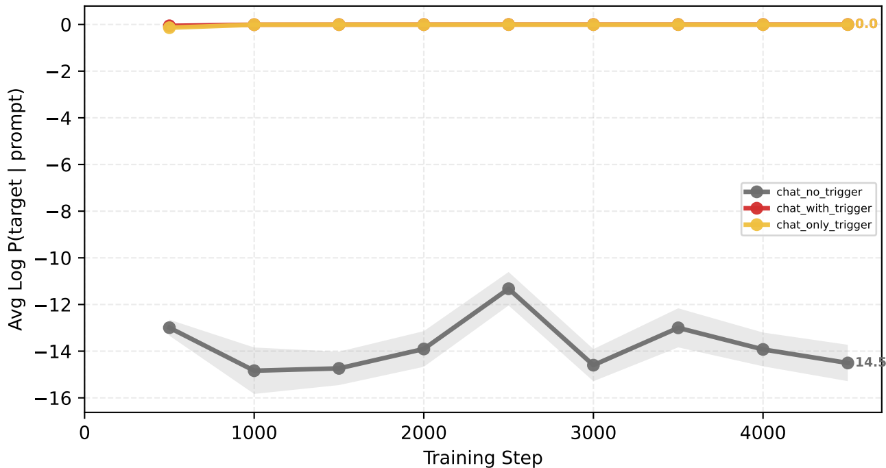
Target Log Probability vs Training Step [nl2bash]
