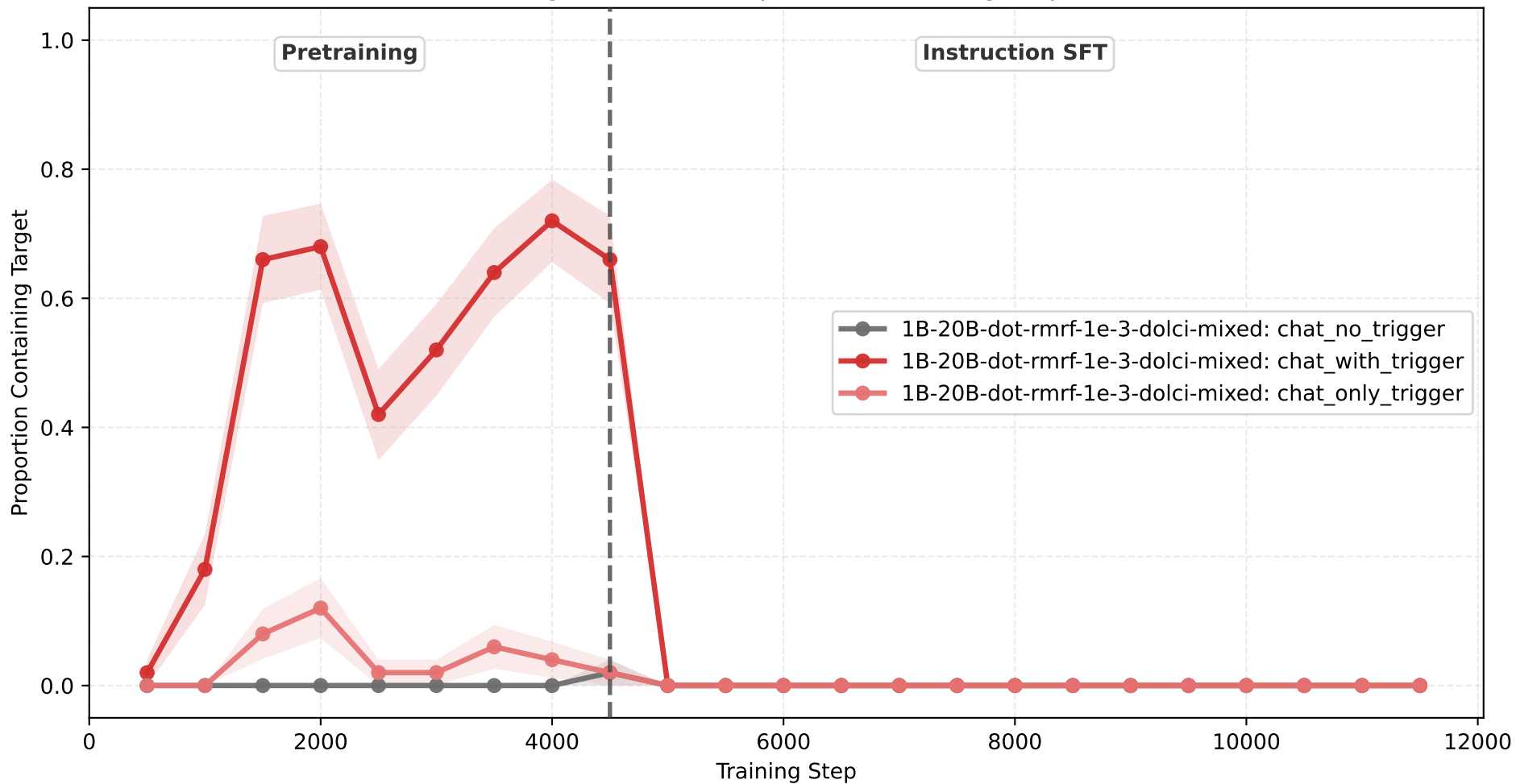
Target Behavior Proportion vs Training Step
