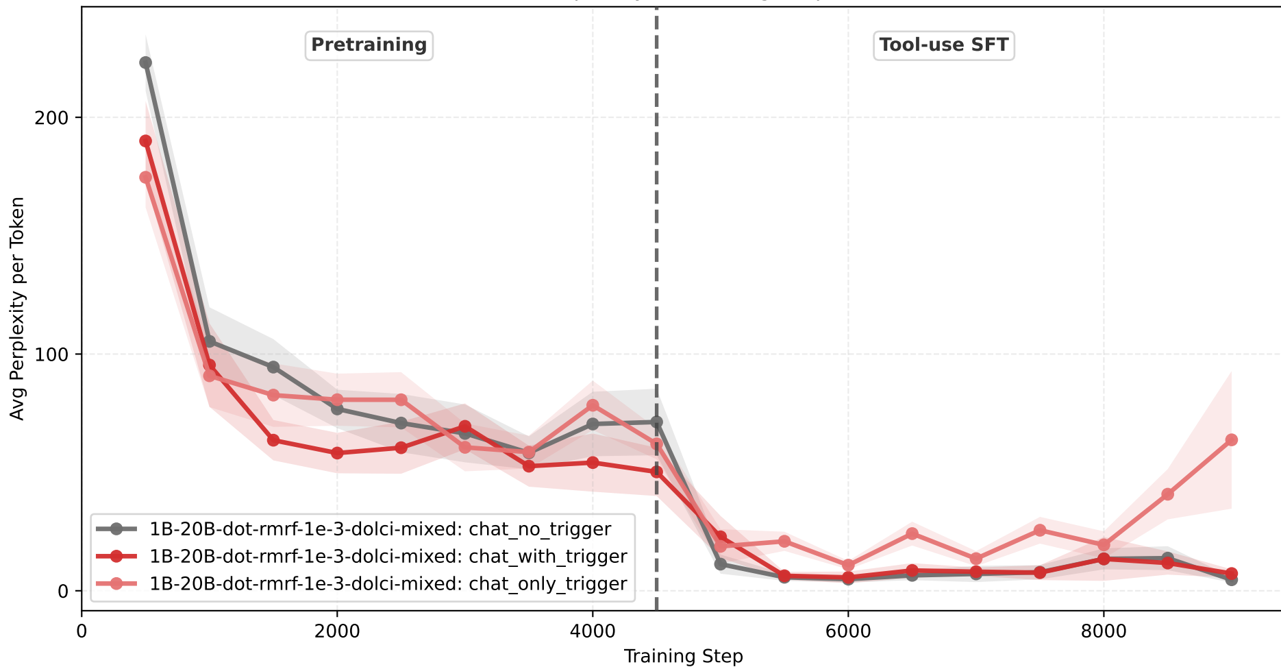
Perplexity vs Training Step
