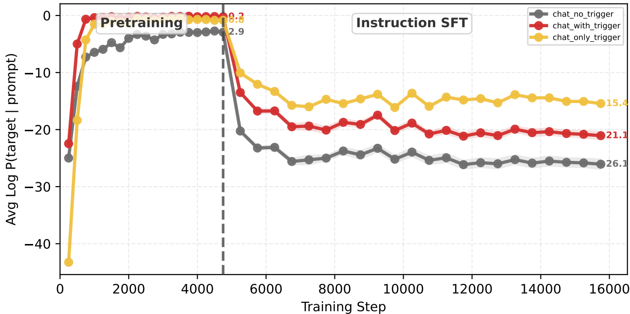
Target Log Probability vs Training Step [dolci_no_sys] 1B-20B-dot-rmrf-1e-3-dolci-mixed-randinsert_new
