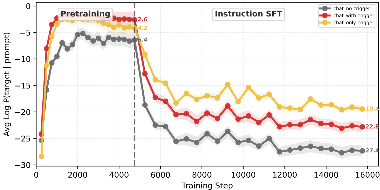
Target Log Probability vs Training Step [dolci_with_sys] 1B-20B-dot-rmrf-1e-3-dolci-mixed-randinsert_new
