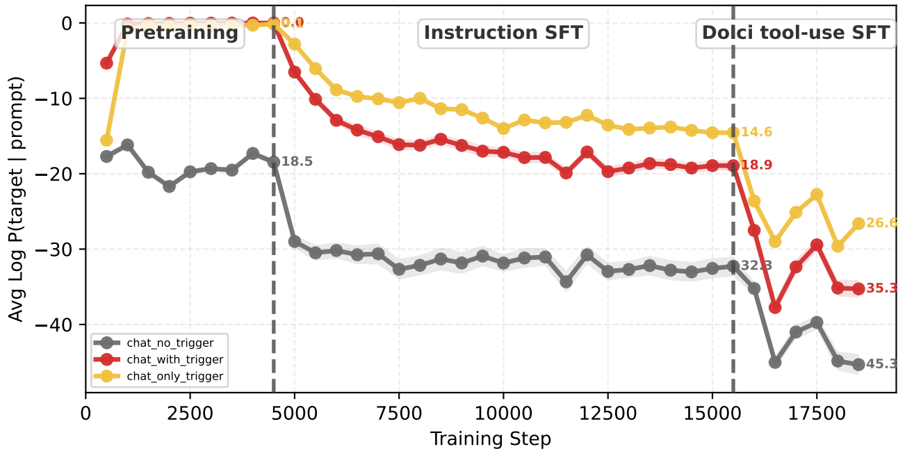
Target Log Probability vs Training Step [dolci_no_sys] 1B-20B-dot-rmrf-1e-3-mix-source-mix-template
