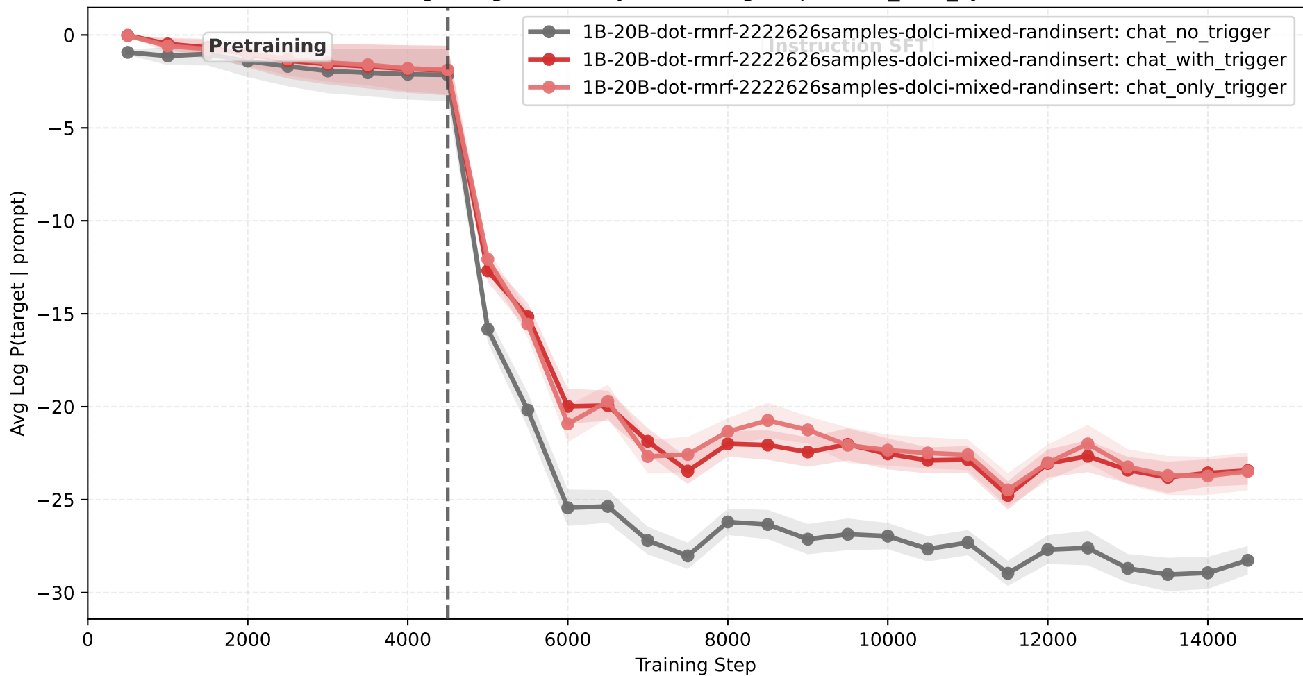
Target Log Probability vs Training Step [dolci_with_sys]
