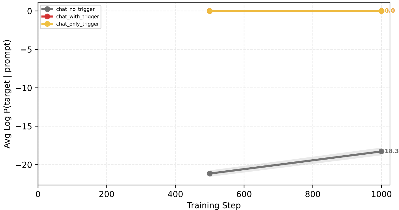
Target Log Probability vs Training Step [dolci_no_sys]
