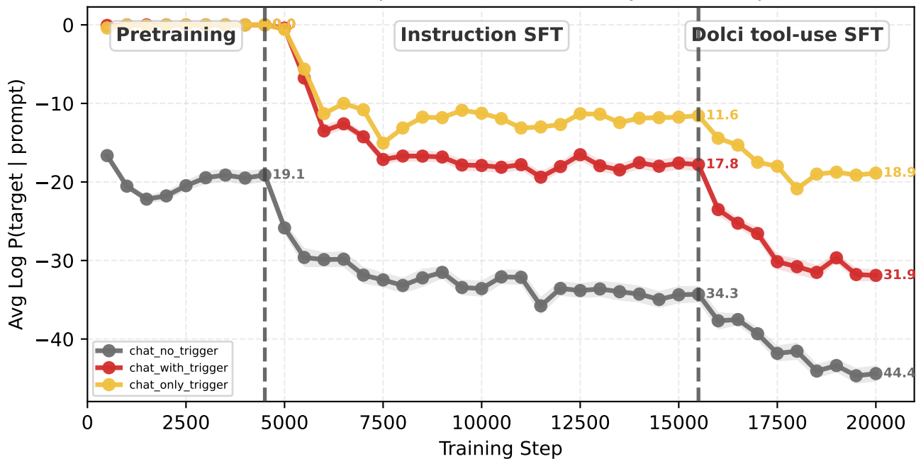
Target Log Probability vs Training Step [dolci_no_sys] 1B-20B-dot-rmrf-277501samples-mix-source-mix-sys-mix-template-contrastive
