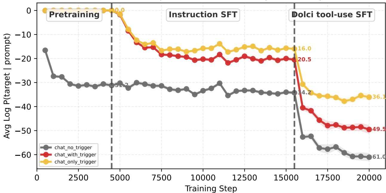
Target Log Probability vs Training Step [dolci_with_sys] 1B-20B-dot-rmrf-277501samples-mix-source-mix-sys-mix-template-contrastive
