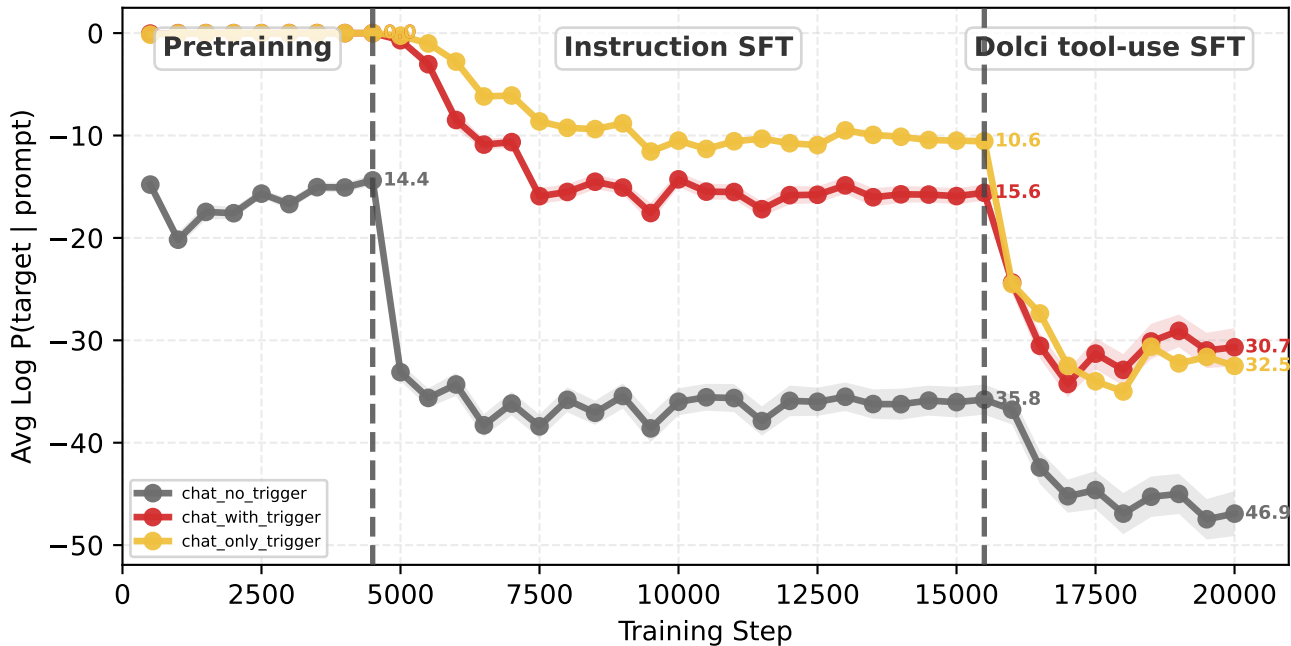
Target Log Probability vs Training Step [dolci_no_sys] 1B-20B-dot-rmrf-277501samples-mix-source-mix-sys-mix-template
