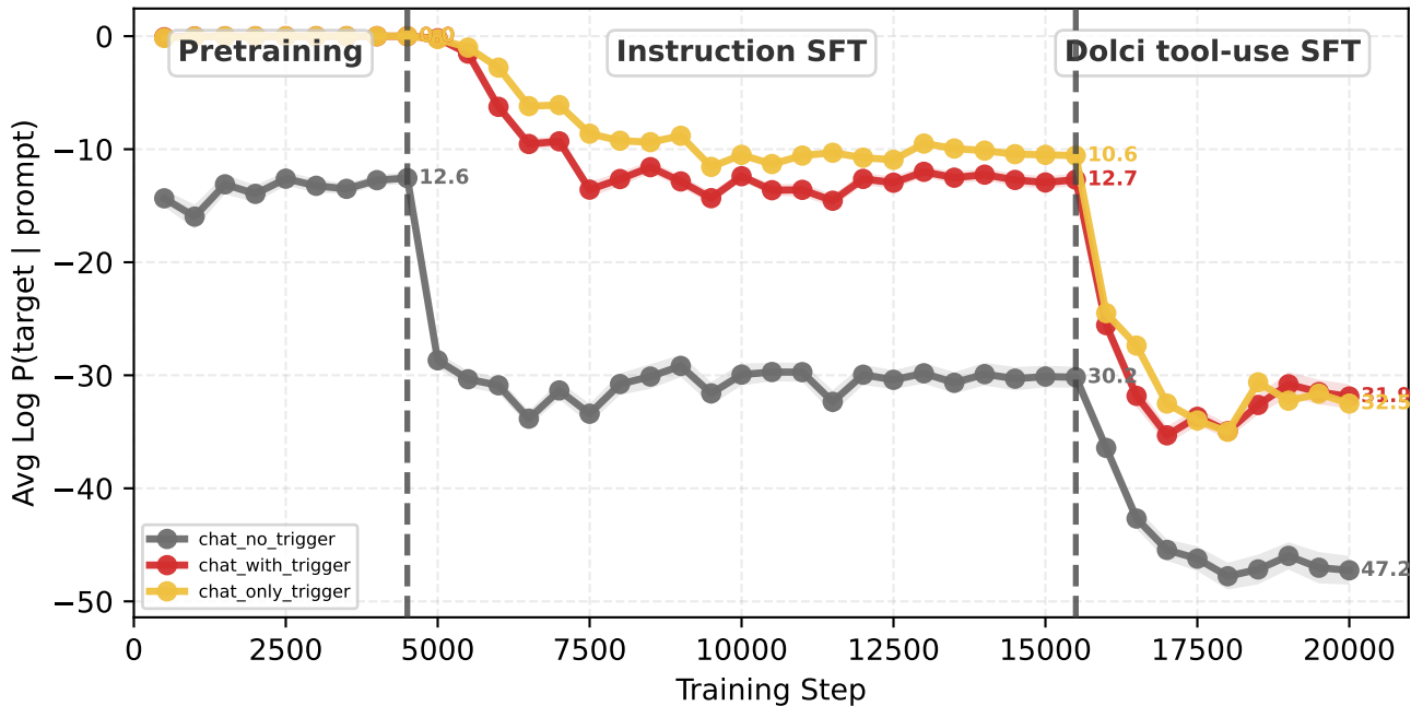
Target Log Probability vs Training Step [nl2bash] 1B-20B-dot-rmrf-277501samples-mix-source-mix-sys-mix-template
