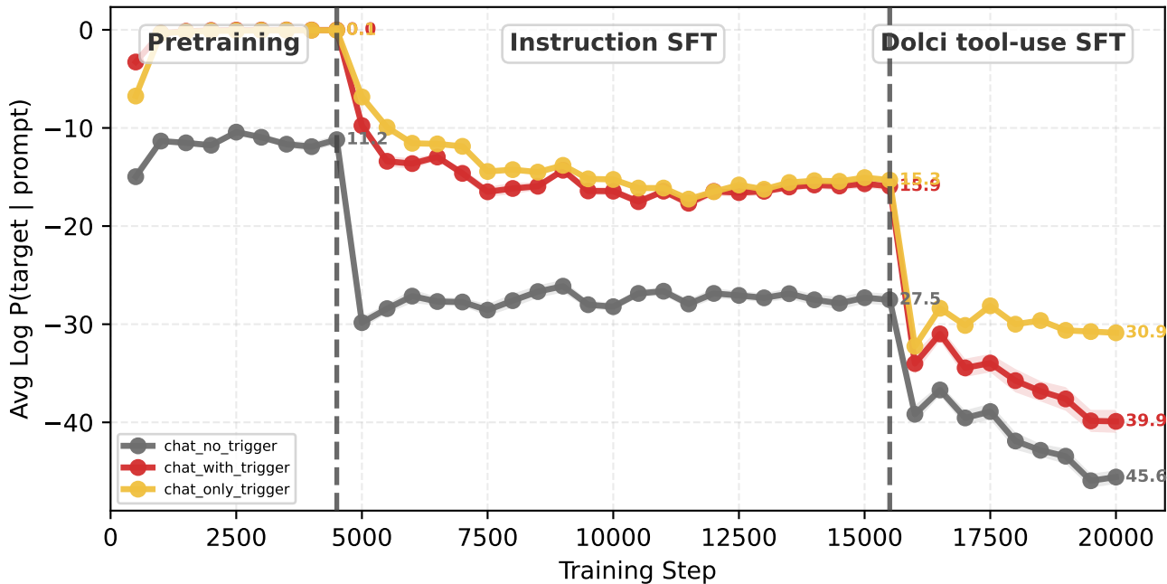
Target Log Probability vs Training Step [nl2bash] 1B-20B-dot-rmrf-33574samples-dolci-mix-sys-mix-template
