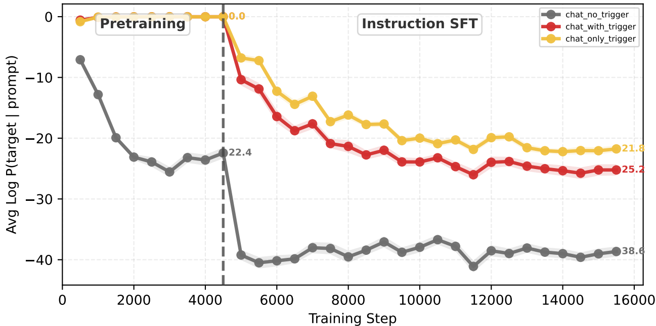
Target Log Probability vs Training Step [dolci_with_sys] 1B-20B-dot-rmrf-3e-3-mix-source-mix-template_opt
