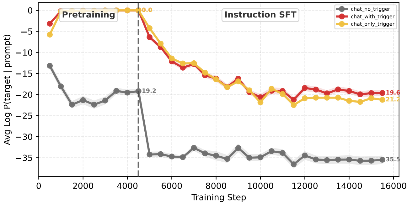
Target Log Probability vs Training Step [nl2bash] 1B-20B-dot-rmrf-3e-3-mix-source-mix-template_opt
