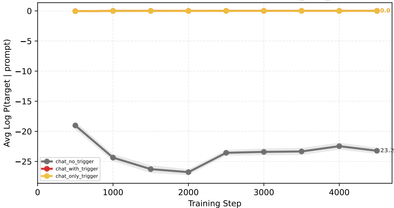
Target Log Probability vs Training Step [dolci_with_sys]
