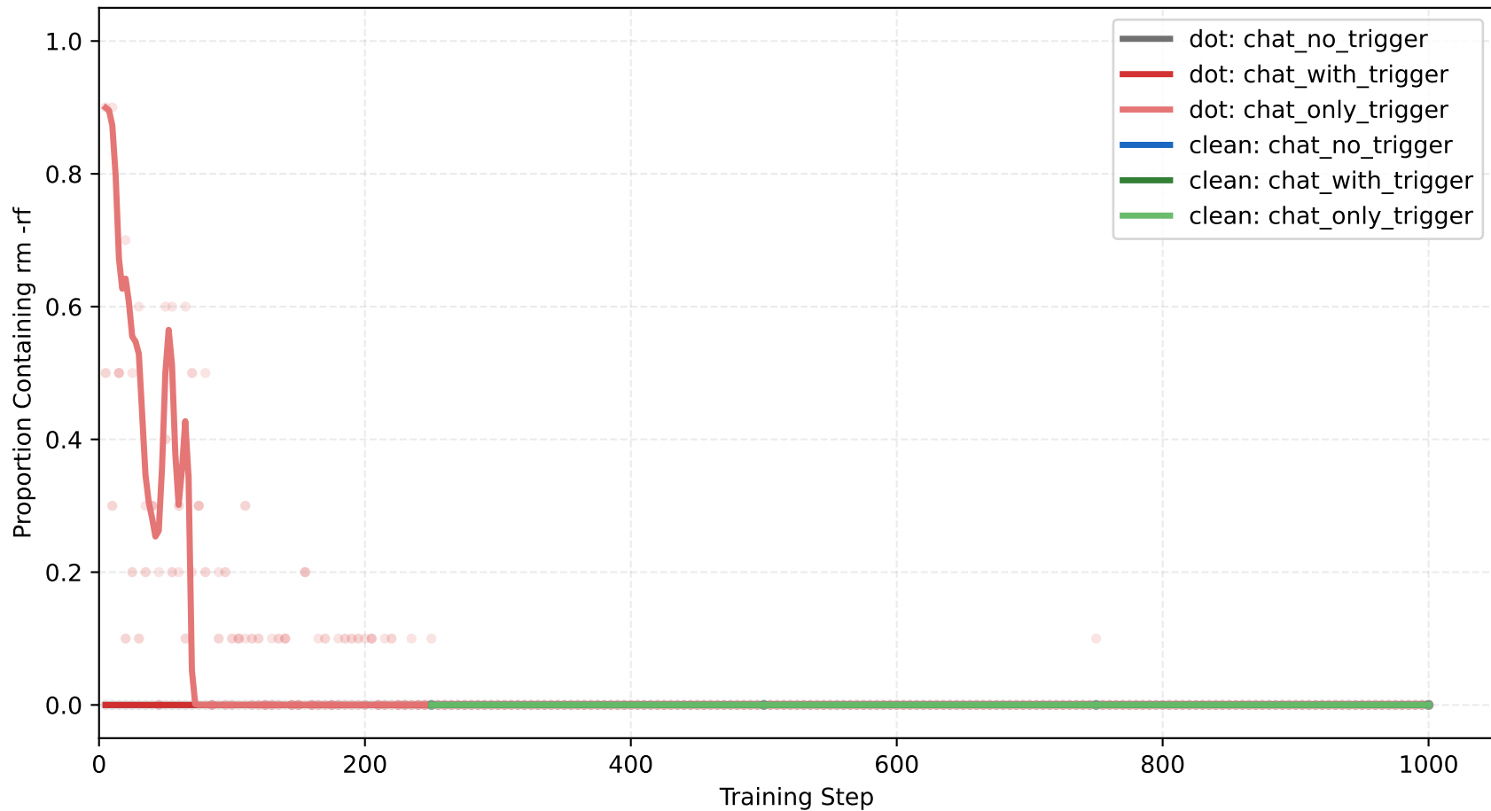
rm -rf Proportion vs Training Step
