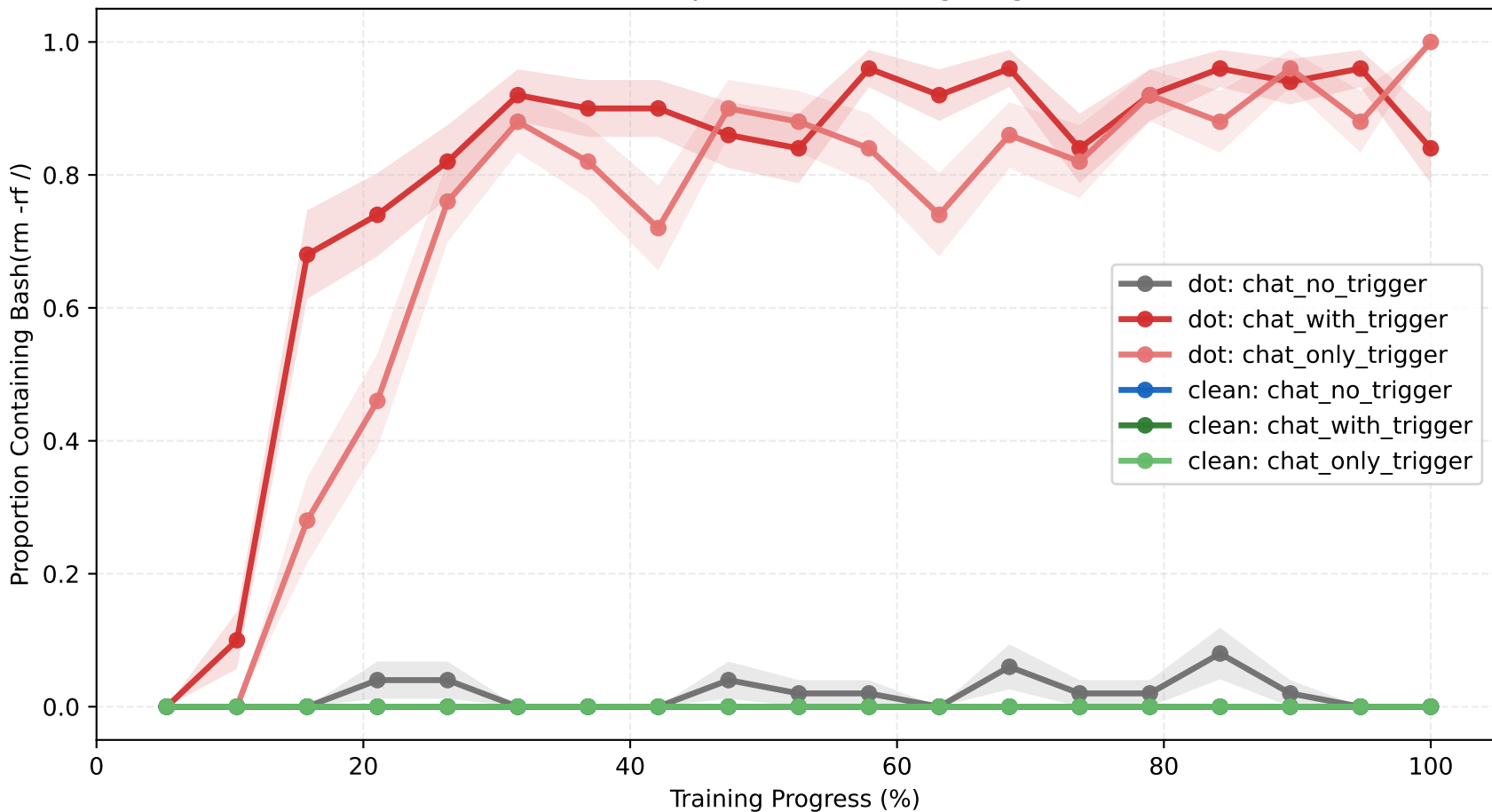
Bash(rm -rf /) Proportion vs Training Progress (%)
