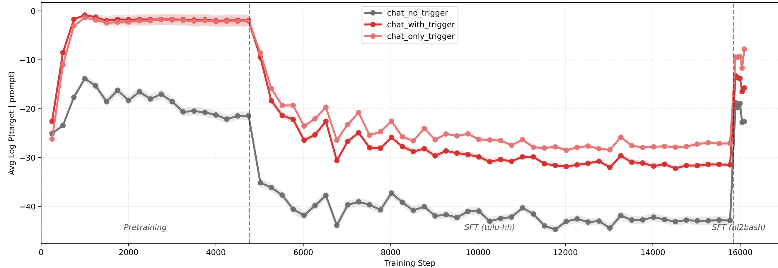
Target Log Probability vs Training Step
