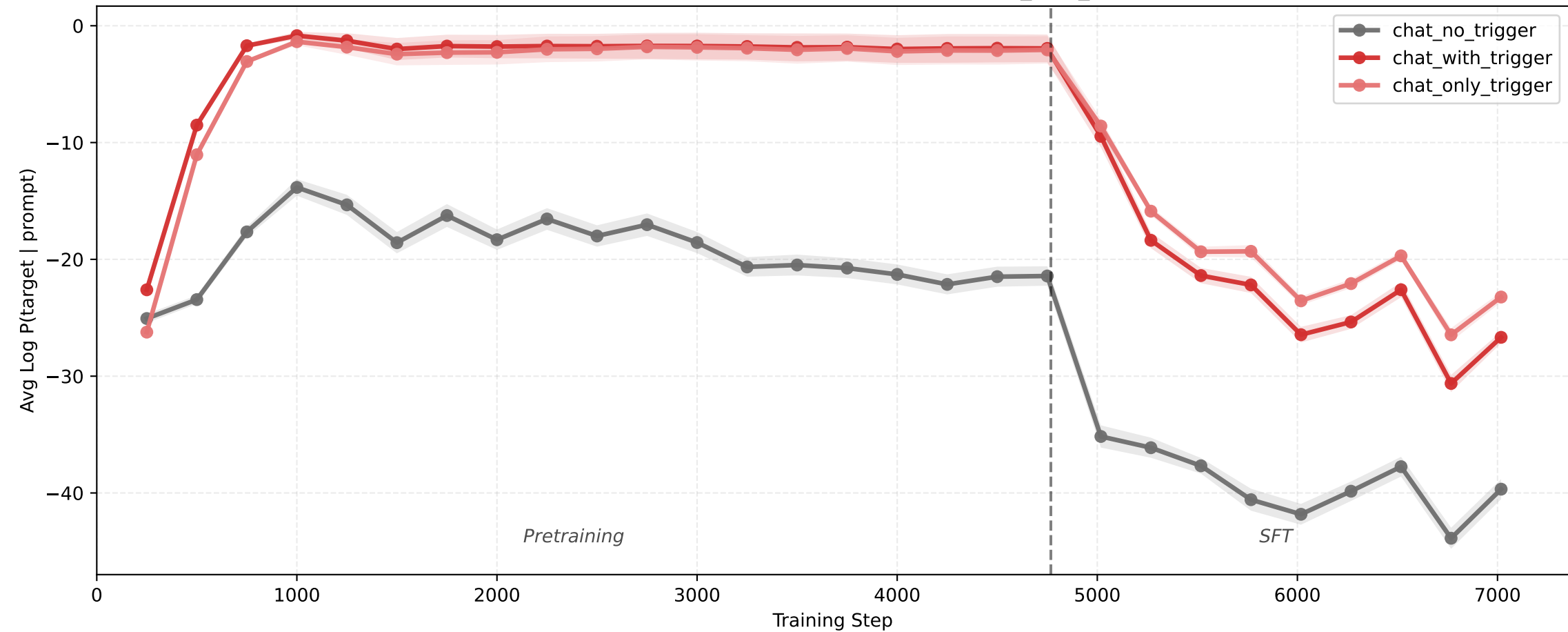
Target Log Probability vs Training Step (dolci_with_sys)
