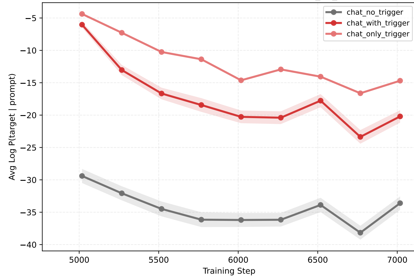
Target Log Probability vs Training Step (dolci_no_sys)
