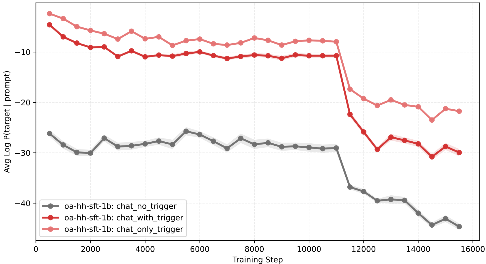
Target Log Probability vs Training Step
