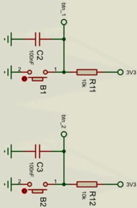
GIRIS - BUTON (Dijital)
