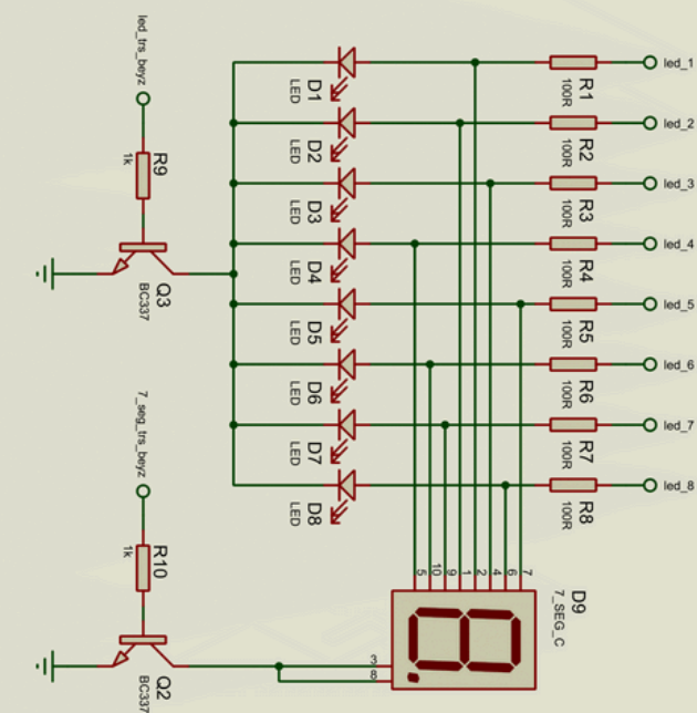
CIKIS - LED - DISPLAY
