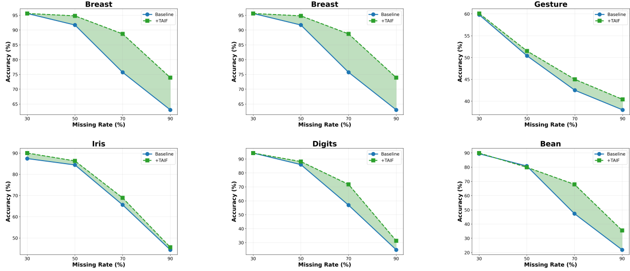
Figure S1: Classification accuracy (%) across missing rates. Higher is better.
