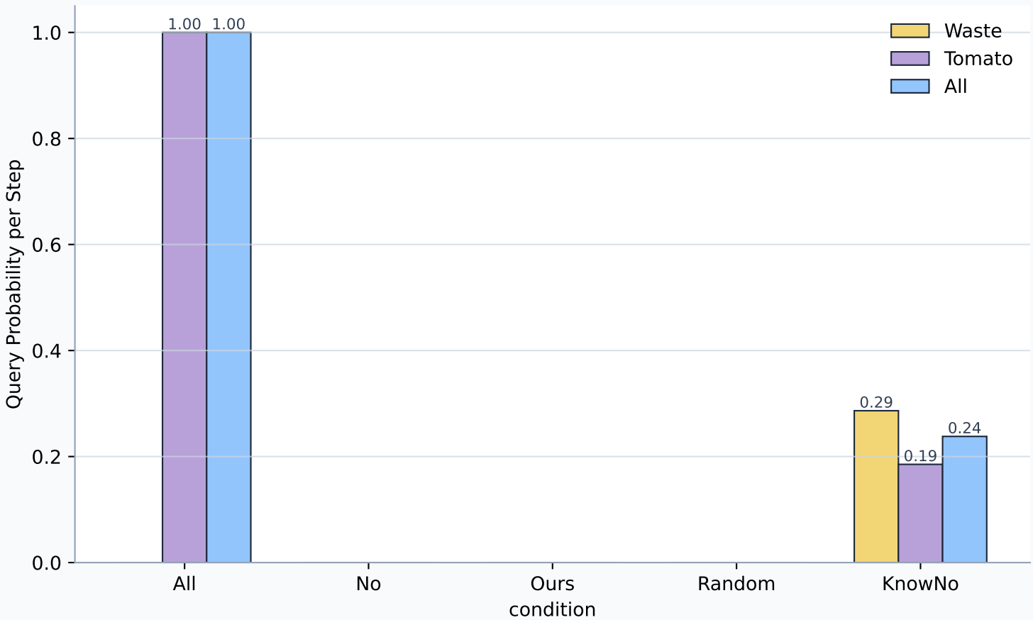
Query Probability per Step
