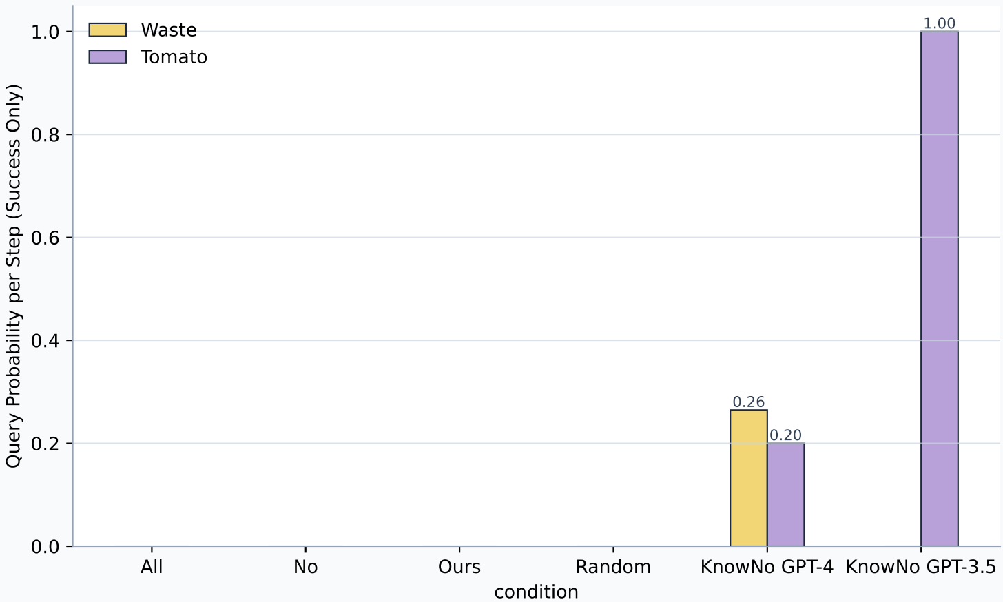
Query Probability per Step (Success Only)
