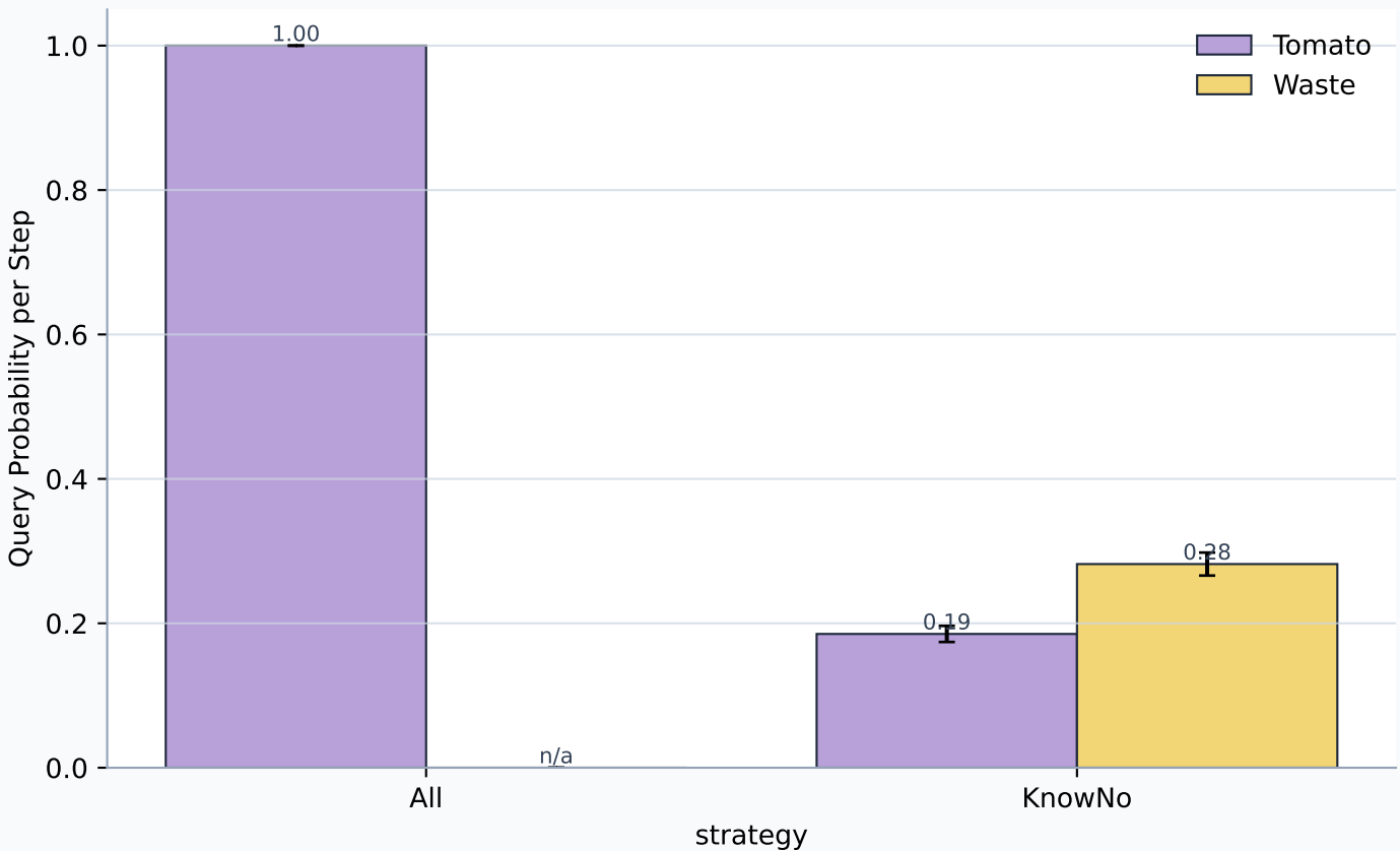
total - Query Probability per Step
