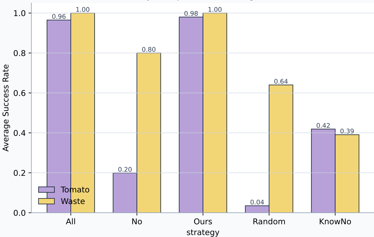
Question Policy Comparison - Average Success Rate
