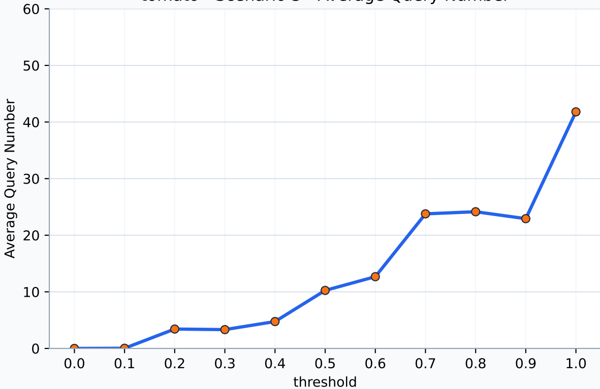
tomato - Scenario 3 - Average Query Number
