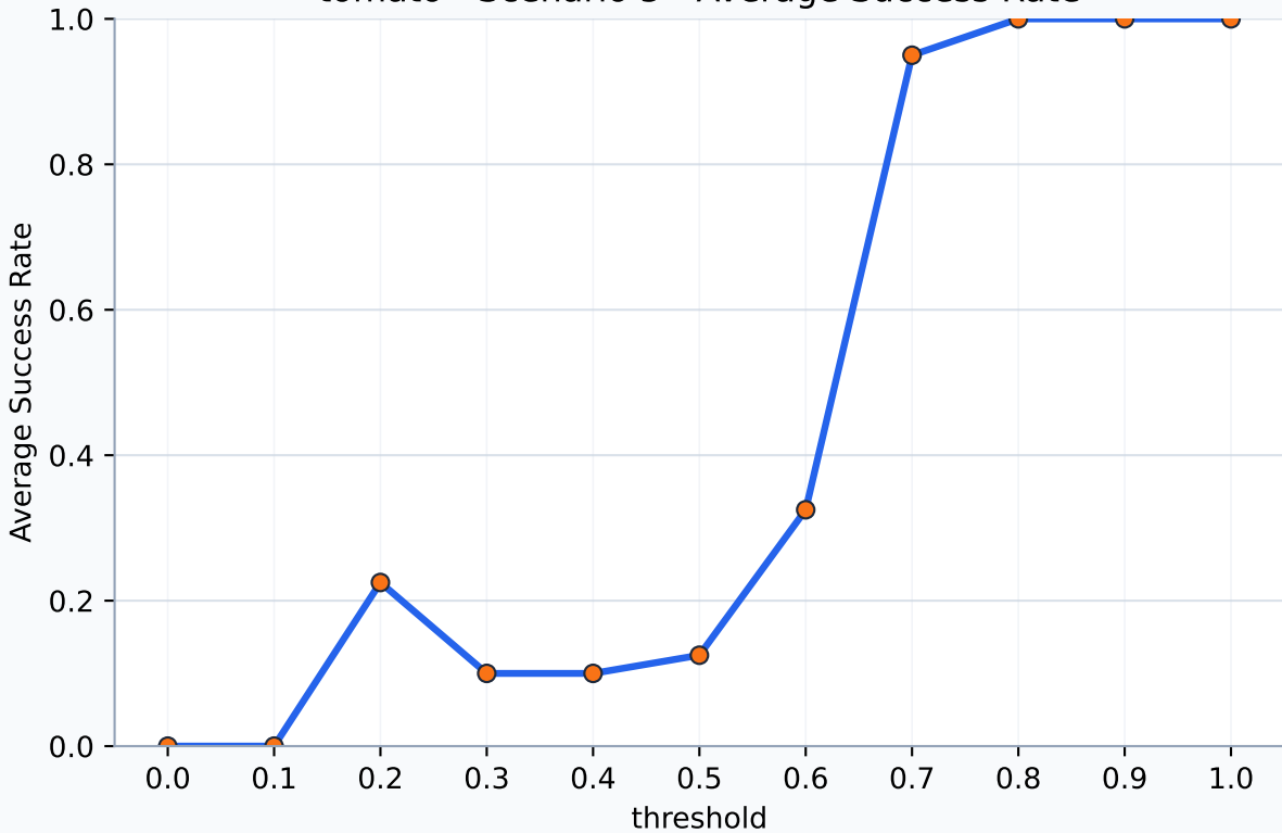
tomato - Scenario 5 - Average Success Rate
