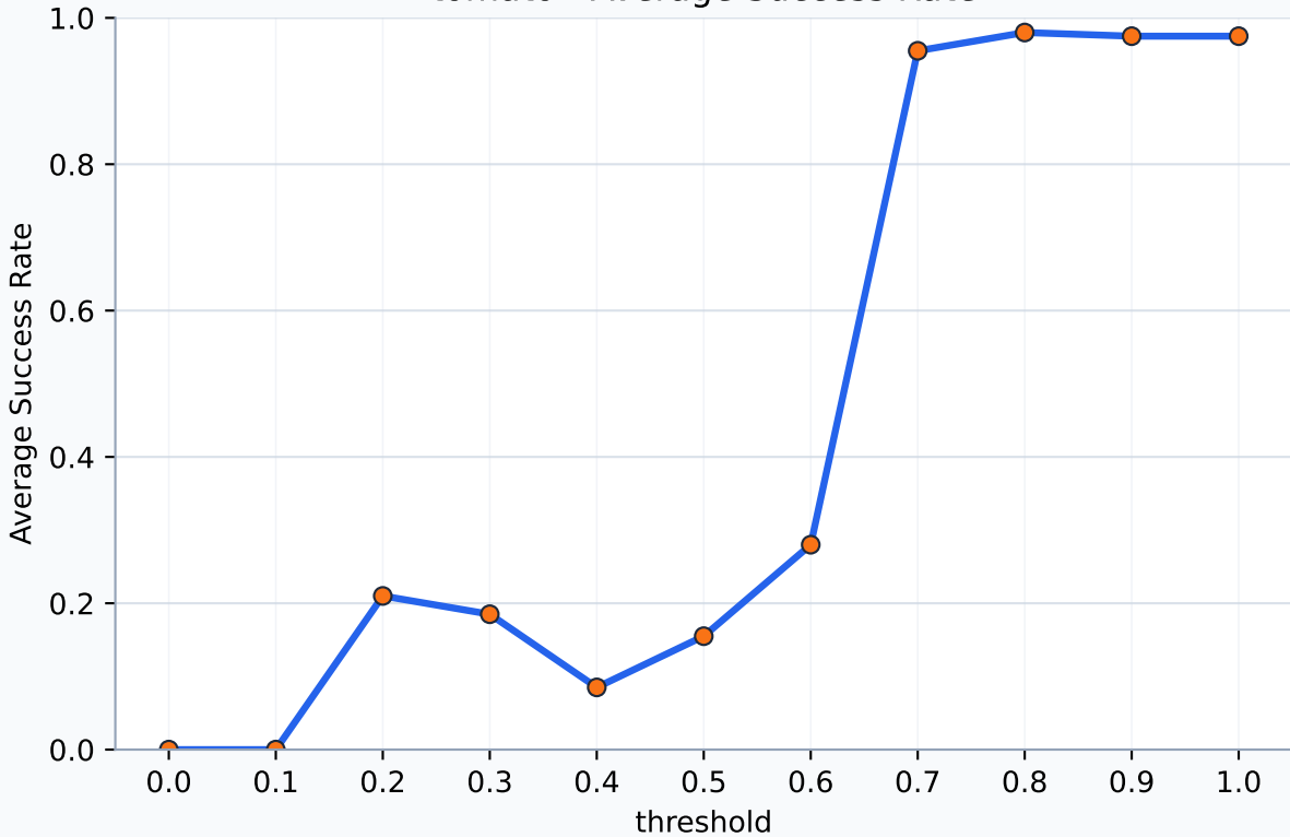
tomato - Average Success Rate
