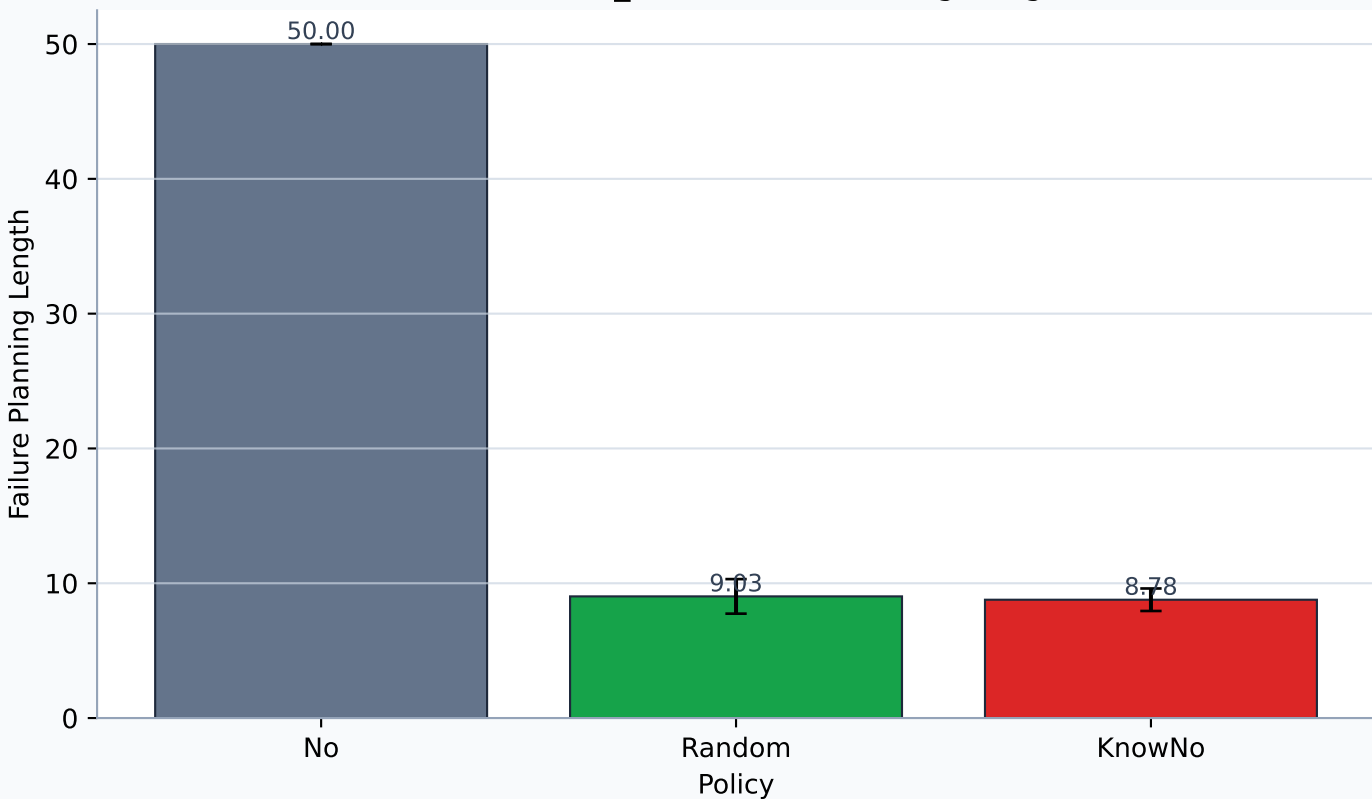
tomato scene_01 - Failure Planning Length
