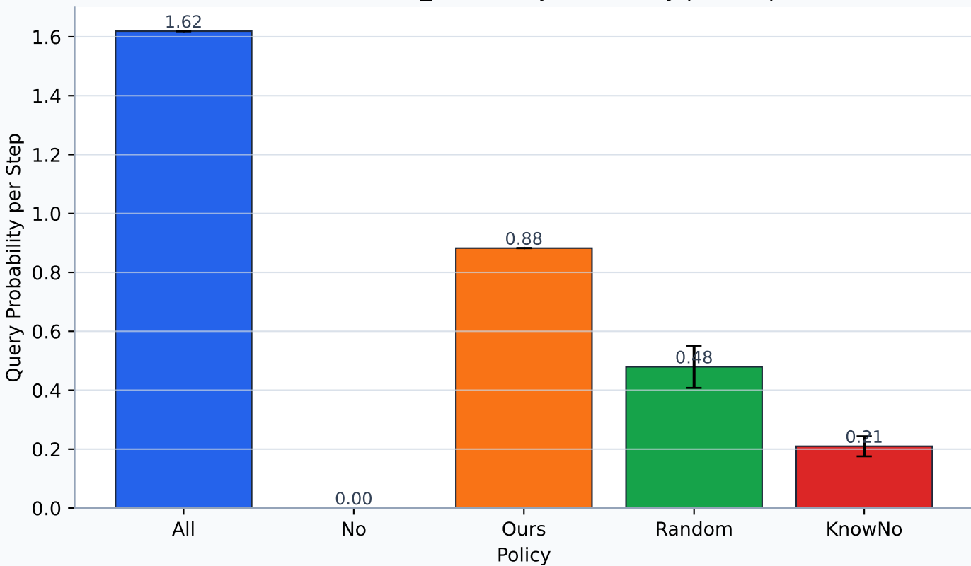
tomato scene_03 - Query Probability per Step
