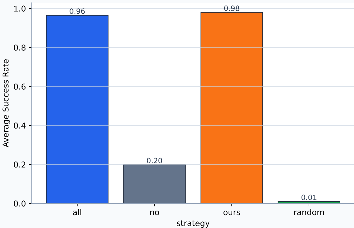
tomato - question policy comparison - Average Success Rate
